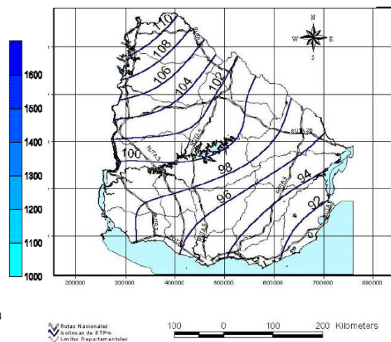
Figura 5.6 – Isolinias de ETP media de Penman (mm/mes)
